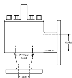
Closed Vent - Pressure Only (Flanged Style Only)
